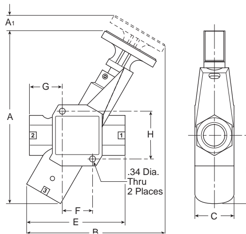
EZ Series, 3/4" Exhaust Port Inches (mm)
