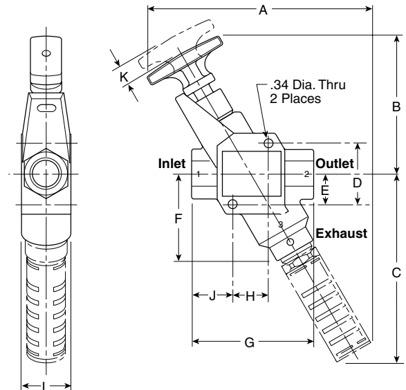
EZ Series Valve shown with optional ES Series Silencer. For more information refer to Section D.
