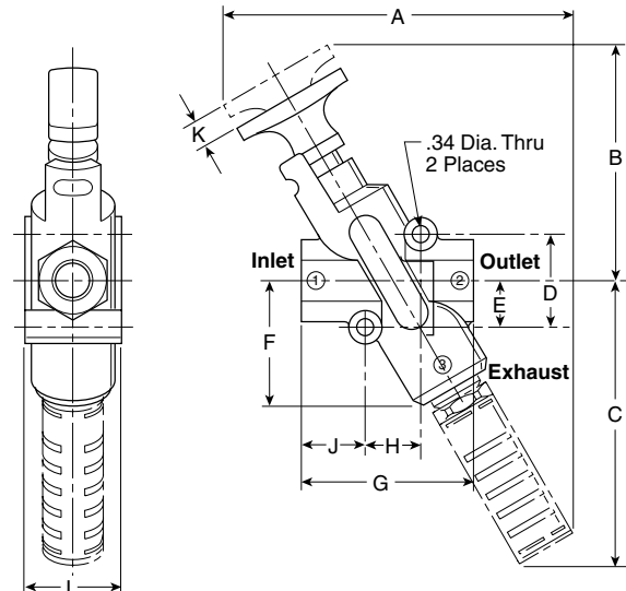
LV Series Valve shown with optional ES Series Silencer. For more information refer to Section D.
